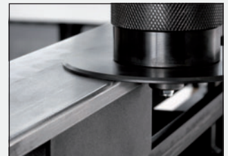
Radius R 2.5 mm
